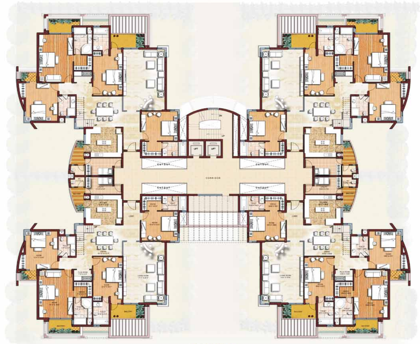
TYPE B PENTHOUSE LOWER LEVEL PLAN 4 BEDROOM + Utility SALEABLE AREA = 3700 sq.ft.
